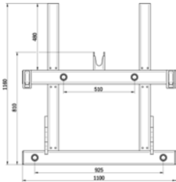
Version with extension and 4 round bale tines (2 tines as standard)
