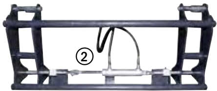
Quick exchange frame, hydraulic locking mechanism
